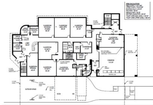
FIRST FLOOR PLAN SCALE: 1/8" = 1'-0"
